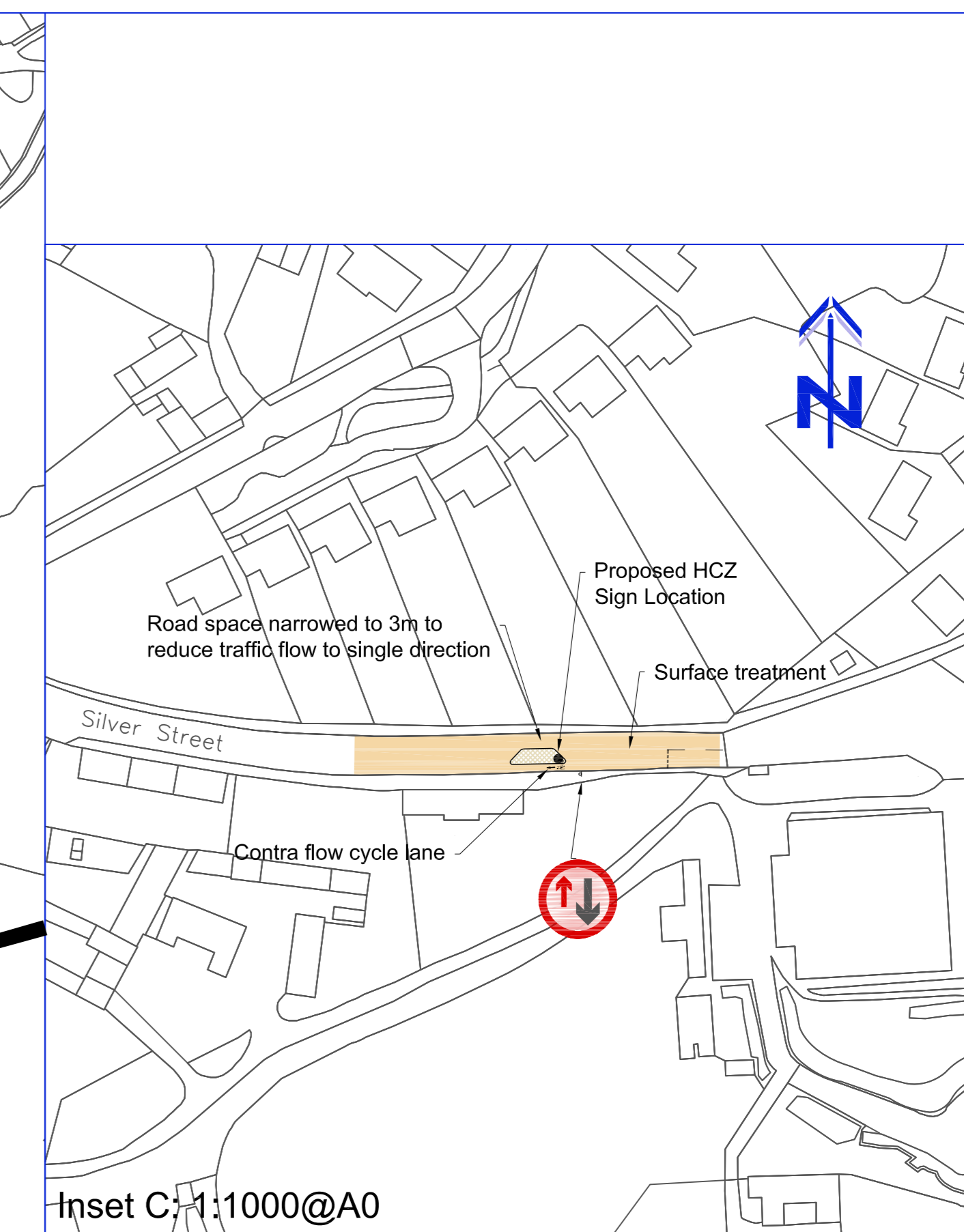
Inset C: 1:1000@A0
