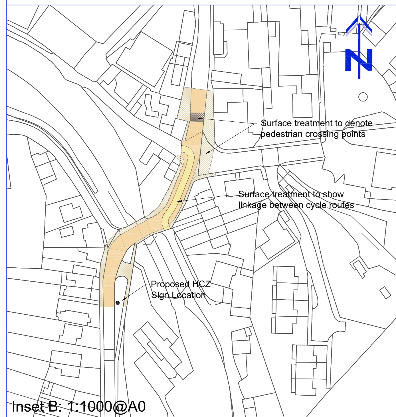
Inset B: 1:1000@A0
